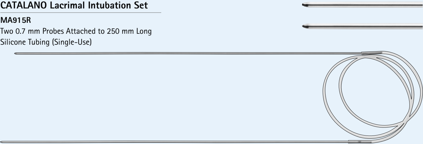
MA915R
